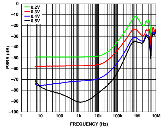
Figure 13. LDO PSRR vs. Frequency, V_{PVOUT2} = 3.3 V , I_{LOAD2} = 1 A at Various LDO Headroom Voltages
