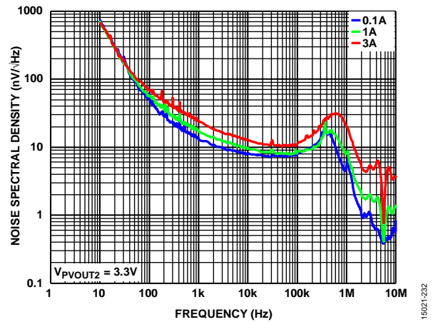
Figure 14. LDO Noise Spectral Density vs. Frequency, V_{PVOUT2} = 3.3 V at Various LDO Load Currents
