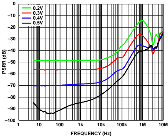
Figure 10. LDO PSRR vs. Frequency, V_{PVOUT2} = 1.3 V , I_{LOAD2} = 1 A at Various LDO Headroom Voltages
