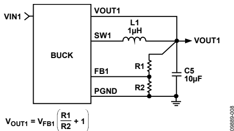
Figure 47. BUCK1 External Output Voltage Setting
