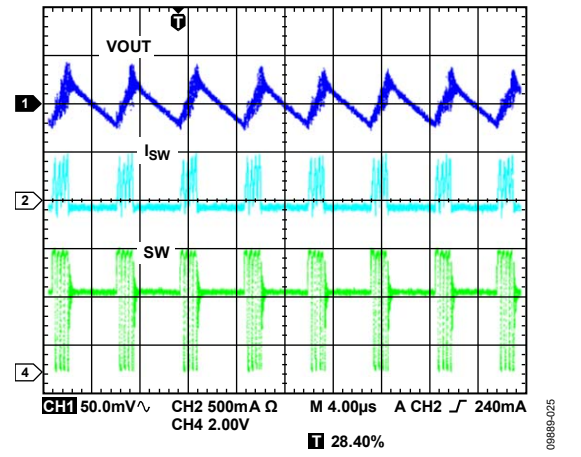
Figure 19. Typical Waveforms, V_{OUT1} = 3.3V , I_{OUT1} = 30mA , Auto Mode
