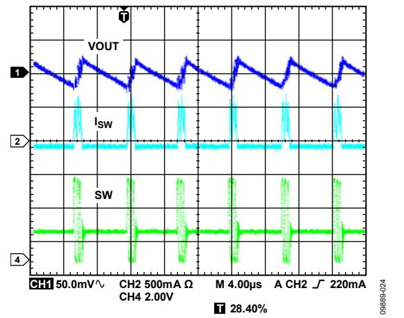
Figure 20. Typical Waveforms, V_{OUT2} = 1.8V , I_{OUT2} = 30mA , Auto Mode
