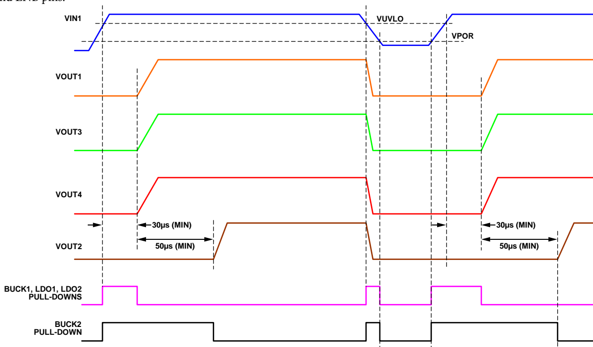
Figure 44. Regulators Sequencing on the ADP5033 ( ENx = VINx )
