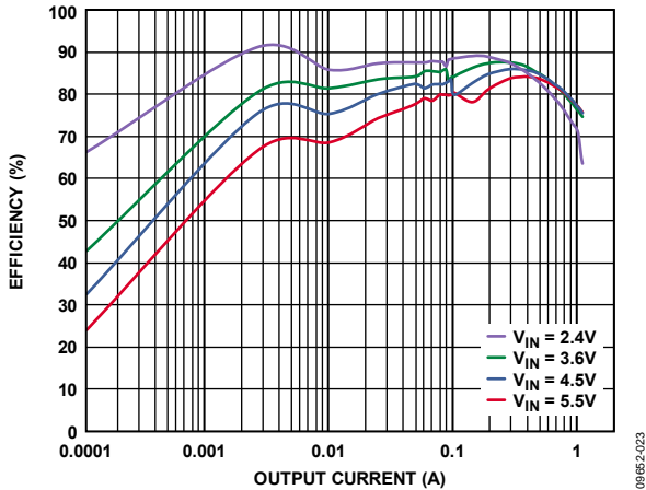
Figure 23. Buck Efficiency vs. Load Current, Across Input Voltage, V_{OUT1} = 1.2\text{ V} , Auto Mode
