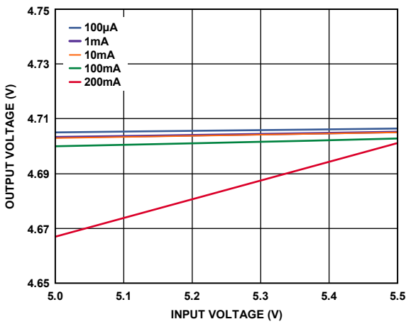
Figure 70. LDO1, LDO2 Line Regulation Across Input Voltage, V_{OUT} = 4.7 V
