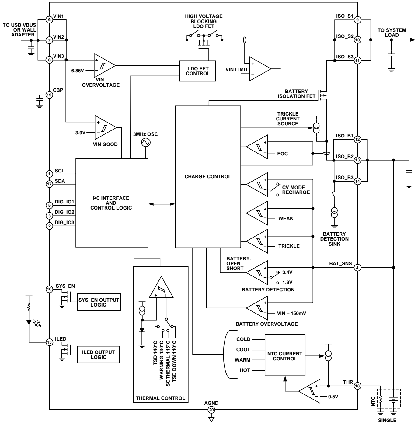
Figure 29. Block Diagram
