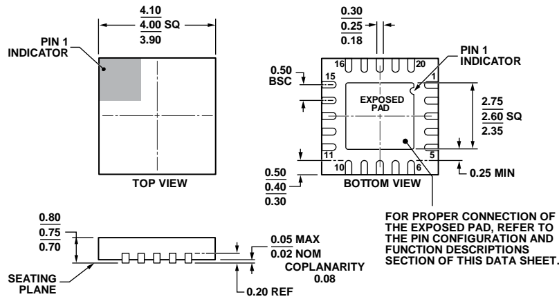
COMPLIANT TO JEDEC STANDARDS MO-220-WGGD. Figure 42. 20-Lead Lead Frame Chip Scale Package [LFCSP_WQ] 4 mm × 4 mm Body, Very Very Thin Quad (CP-20-8) Dimensions shown in millimeters
