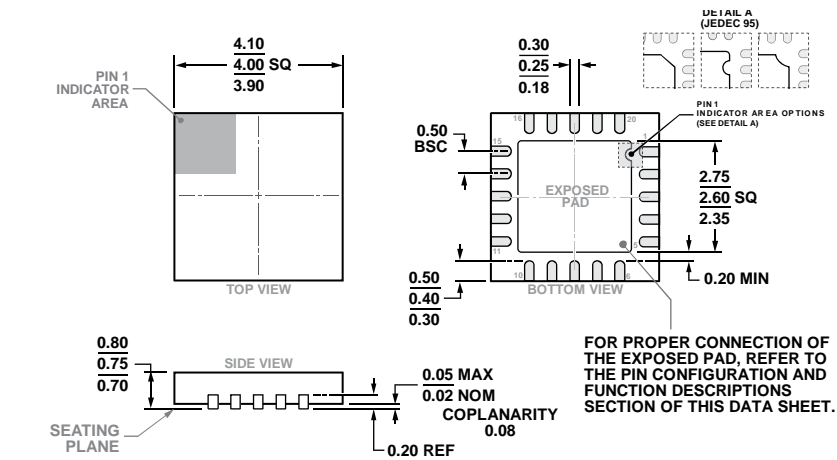
Figure 52. 20-Lead Lead Frame Chip Scale Package [LFCSP] 4 mm x 4 mm Body and 0.75 mm Package Height (CP-20-8)
