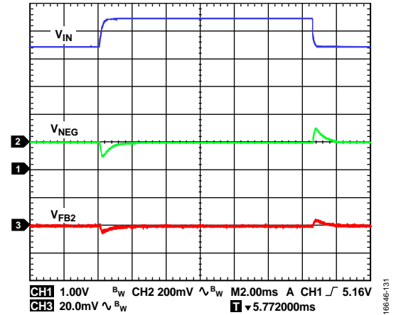
Figure 31. Inverting Regulator Line Transient, V_{IN} = 4.5\text{ V} to 5.5\text{ V} Step, V_{NEG} = -15\text{ V} , R_{LOAD2} = 300\ \Omega , f_{SW} = 2.4\text{ MHz} , T_A = 25^\circ\text{C}
