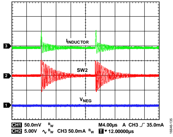
Figure 36. Inverting Regulator Skip Mode Operation Showing Inductor Current ( I_{INDUCTOR} ), Switch Node Voltage, and Output Ripple, V_{IN} = 5V , V_{NEG} = -5V , I_{LOAD2} = 0mA , f_{SW} = 2.4MHz , T_A = 25^\circ C
