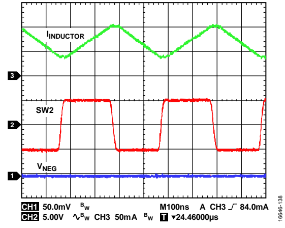
Figure 38. Inverting Regulator Continuous Conduction Mode Operation Showing Inductor Current ( I_{INDUCTOR} ), Switch Node Voltage, and Output Ripple, V_{IN} = 5V , V_{NEG} = -5V , I_{LOAD2} = 35mA , f_{SW} = 2.4MHz , T_A = 25^\circ C
