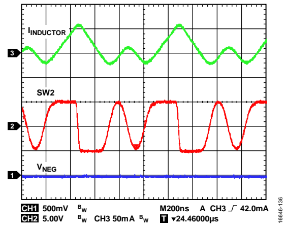
Figure 37. Inverting Regulator Discontinuous Conduction Mode Operation Showing Inductor Current ( I_{INDUCTOR} ), Switch Node Voltage, and Output Ripple, V_{IN} = 5V , V_{NEG} = -5V , I_{LOAD2} = 6mA , f_{SW} = 2.4MHz , T_A = 25^\circ C
