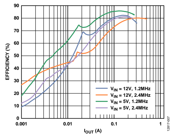
Figure 7. Efficiency vs. Current Load ( I_{OUT} ), V_{IN} = 12V and 5V , V_{OUT} = -15V , T_A = 25^\circ\text{C}
