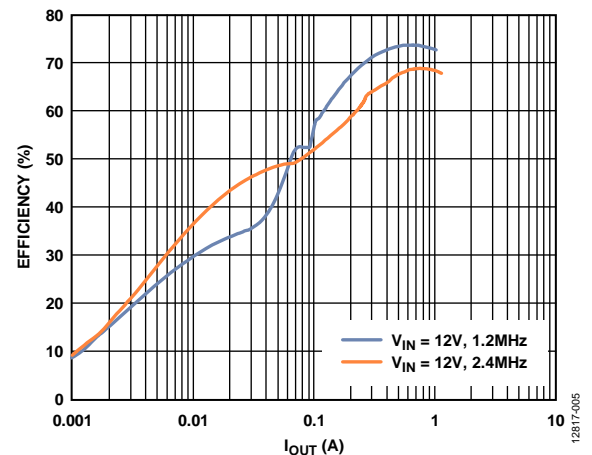
Figure 5. Efficiency vs. Current Load ( I_{OUT} ), V_{IN} = 12V , V_{OUT} = -2.5V , T_A = 25^\circ\text{C}
