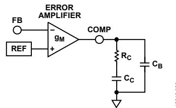
Figure 26. Compensation Components
