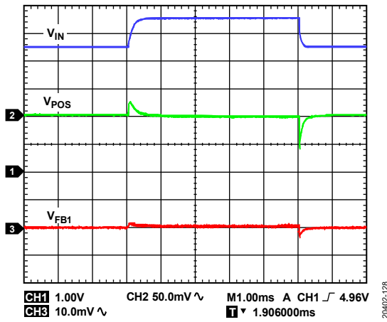
Figure 28. Boost Regulator Line Transient, V_{IN} = 4.5\text{ V} to 5.5\text{ V} Step, V_{POS} = 15\text{ V} , Resistor Load for Boost Regulator ( R_{LOAD1} = 300\ \Omega , f_{SW} = 2.4\text{ MHz} , T_A = 25^\circ\text{C} )
