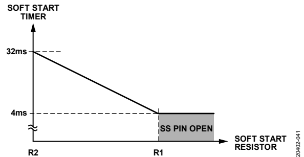
Figure 43. Soft Start Behavior
