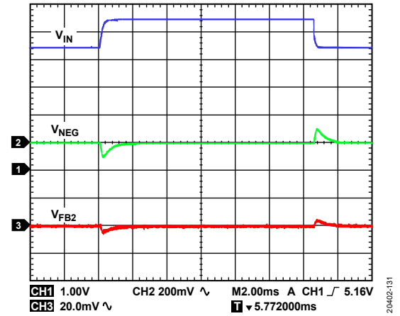
Figure 31. Inverting Regulator Line Transient, V_{IN} = +4.5\text{ V} to +5.5\text{ V} Step, V_{NEG} = -15\text{ V} , Resistor Load for Inverting Regulator ( R_{LOAD2} = 300\ \Omega , f_{SW} = 2.4\text{ MHz} , T_A = 25^\circ\text{C} )
