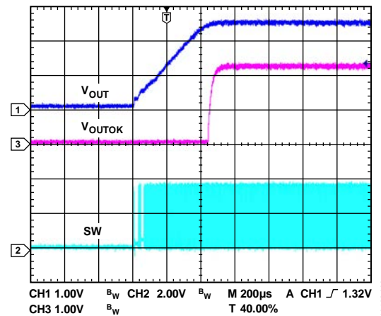
Figure 33. VOUTOK Function
