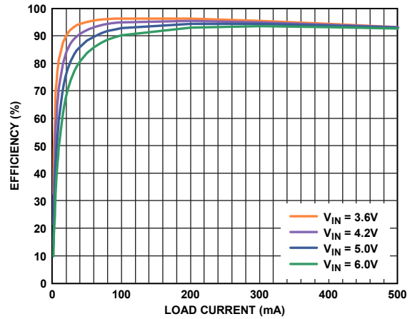
Figure 14. PWM Efficiency vs. Load Current, V_{OUT} = 3.3 V
