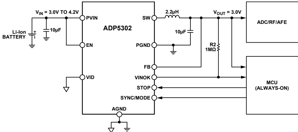
Figure 43. Typical Application Circuit with STOP Switching Functionality
