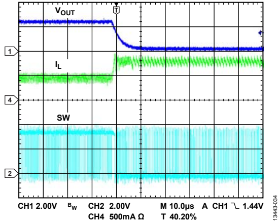
Figure 34. Output Short
