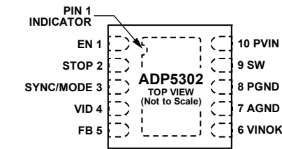
Figure 3. Pin Configuration
