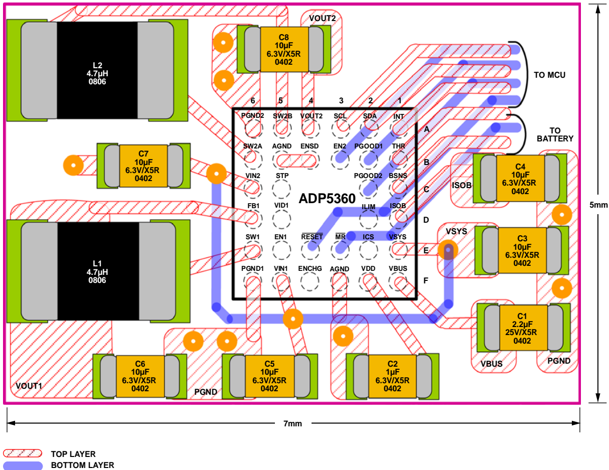
Figure 62. Recommend Layout
