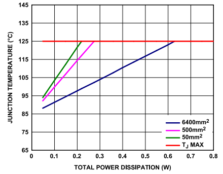
Figure 57. SOIC, T A = 85°C
