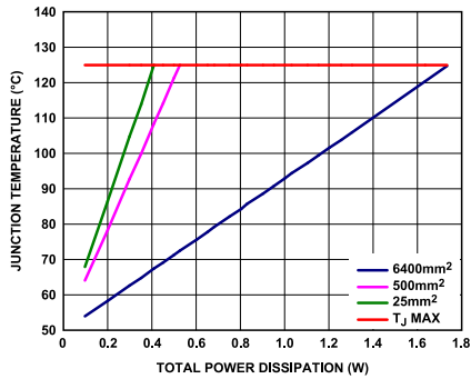
Figure 54. LFCSP, T A = 85°C
