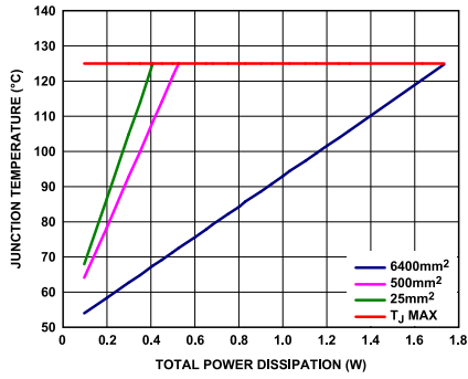
Figure 53. LFCSP, T A = 50°C
