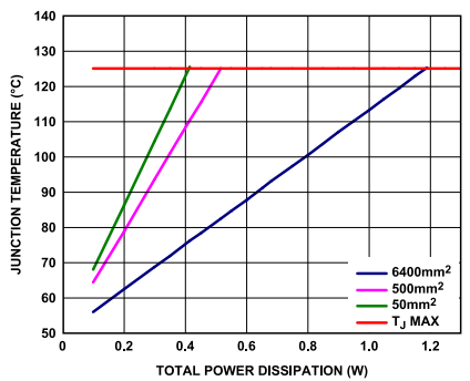
Figure 56. SOIC, T A = 50°C
