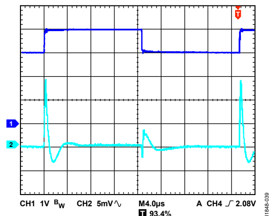
Figure 41. Line Transient Response, I_{LOAD} = 200 \text{ mA} , V_{OUT} = 1.8 \text{ V} , CH1 V_{IN} , CH2 V_{OUT}
