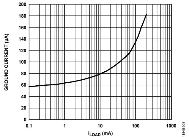
Figure 10. Ground Current vs. Load Current ( I_{LOAD} )
