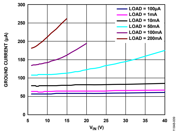
Figure 11. Ground Current vs. Input Voltage ( V_{IN} )
