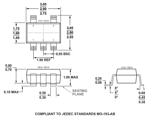
Figure 69. 5-Lead Thin Small Outline Transistor Package [TSOT] (UJ-5) Dimensions shown in millimeters
