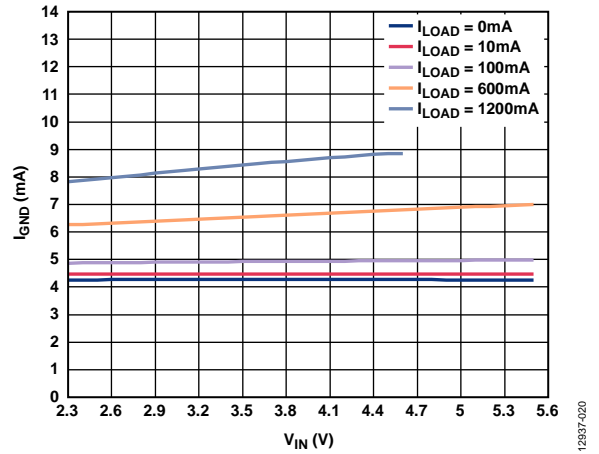
Figure 20. Ground Current ( I_{GND} ) vs. Input Voltage ( V_{IN} ) at Various Loads, V_{OUT} = 1.8\text{ V}
