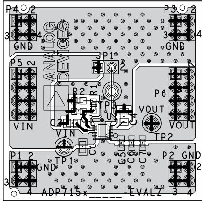
Figure 63. Sample 10-Lead LFCSP PCB Layout
