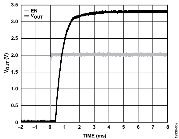
Figure 50. Typical VOUT Response to EN Pin Operation (VEN), VOUT = 3.3 V, VIN = 5 V, CBYP = 1 µF
