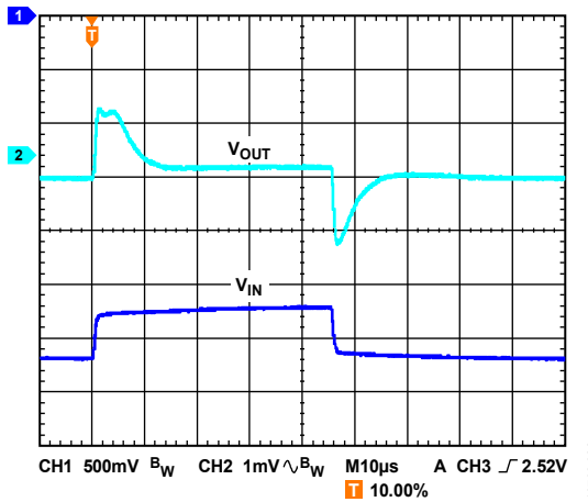
Figure 64. Line Transient Response, 500 mV Step, V_{OUT} = -1.22 V, I_{LOAD} = -10 mA
