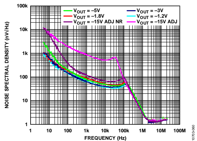
Figure 62. Noise Spectral Density, Various Output Voltages
