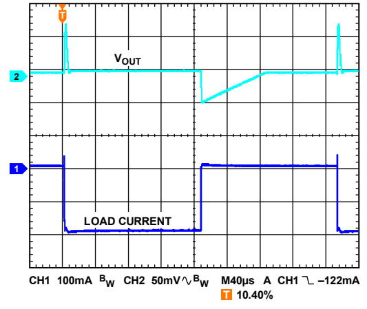
Figure 73. Load Transient Response, V_{OUT} = -1.22V , I_{LOAD} = -1mA to -200mA , Load Step = 1A/\mu s
