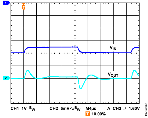
Figure 68. Line Transient Response, 500 mV Step, V_{OUT} = -3 V, I_{LOAD} = -10 mA
