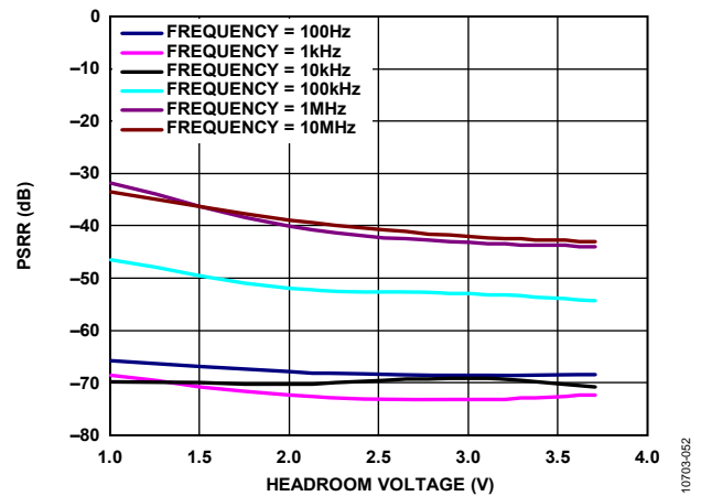
Figure 54. Power Supply Rejection Ratio (PSRR) vs. Headroom Voltage, V_{OUT} = -1.8\text{ V} , Load Current ( I_{LOAD} ) = -200 mA
