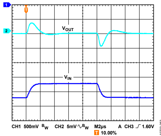
Figure 65. Line Transient Response, 500 mV Step, V_{OUT} = -1.8 V, I_{LOAD} = -200 mA
