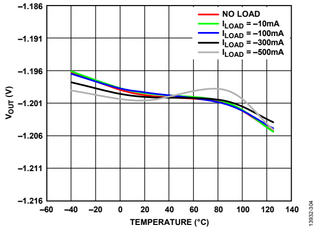
Figure 4. Output Voltage ( V_{OUT} ) vs. Junction Temperature ( T_J ), V_{OUT} = -1.2\text{ V}
