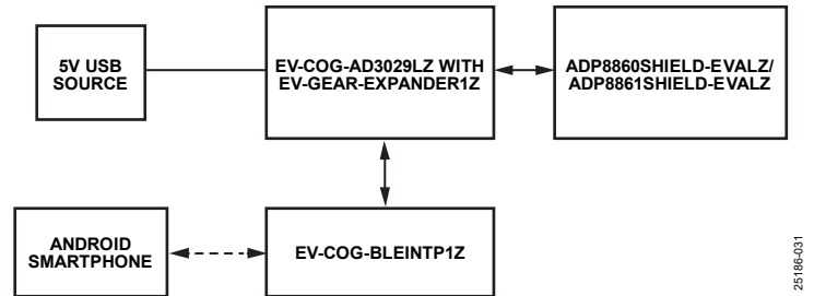
Figure 2. Functional Block Diagram for Android Smartphones
