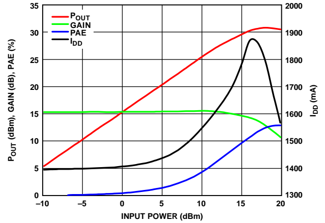
Figure 32. P_{OUT} , Gain, PAE, and I_{DD} vs. Input Power, 20 GHz, V_{DD} = 5\text{ V} , I_{DQ} = 1400\text{ mA}
