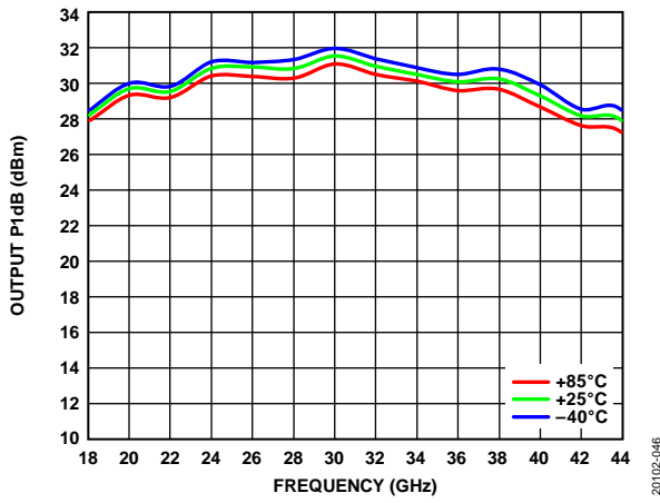
Figure 47. Output P1dB vs. Frequency for Various Temperatures, V_{DD} = 5\text{ V} , Data Measured with Constant I_{DD}
