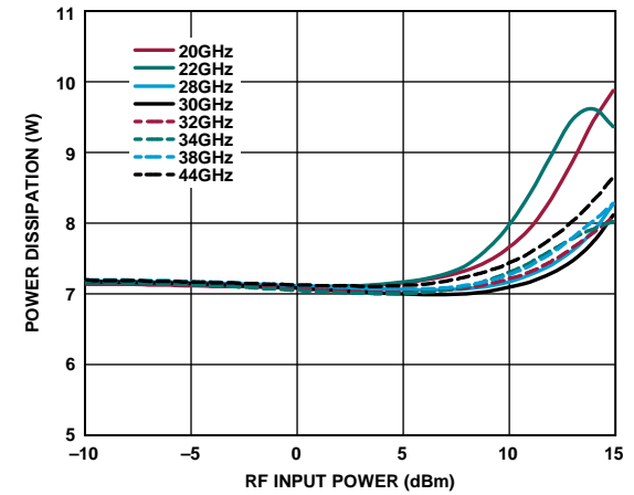
Figure 44. Power Dissipation vs. RF Input Power at T_A = 85^\circ\text{C} , V_{DD} = 5\text{ V} , I_{DQ} = 1400\text{ mA}
