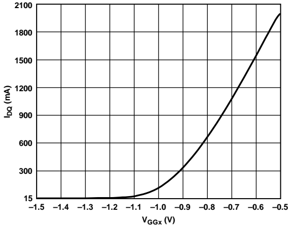
Figure 40. I_{DQ} vs. V_{GGx}
