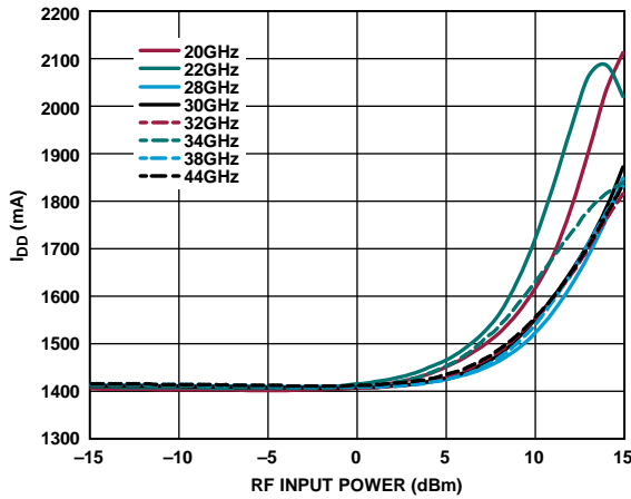
Figure 41. I_{DD} vs. RF Input Power at Various Frequencies, V_{DD} = 5\text{ V} , I_{DQ} = 1400\text{ mA}
