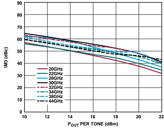
Figure 43. IM3 vs. P_{OUT} per Tone, V_{DD} = 5\text{ V} , I_{DQ} = 1400\text{ mA}
