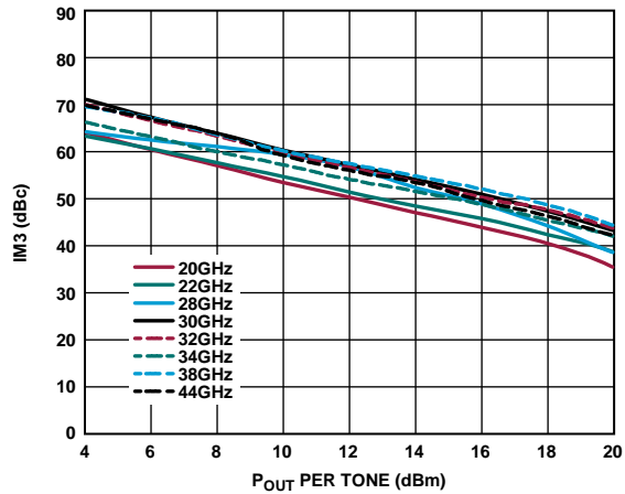
Figure 42. Third-Order Intermodulation Distortion (IM3) vs. P_{OUT} per Tone, V_{DD} = 4\text{ V} , I_{DQ} = 1400\text{ mA}
