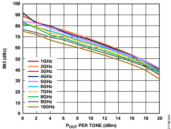
Figure 44. IM3 vs. P_{OUT} per Tone for Various Frequencies, Self Biased Mode, V_{DD} = 12 V, V_{GG1} = GND
