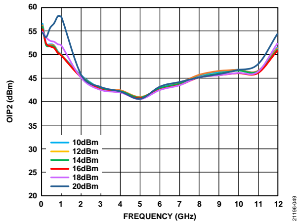
Figure 49. OIP2 vs. Frequency for Various P_{OUT} per Tone, Self Biased Mode, V_{DD} = 12 V, V_{GG1} = GND
