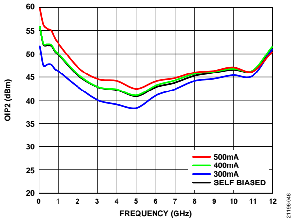
Figure 46. OIP2 vs. Frequency for Various I_{DQ} , Externally Biased Mode, V_{DD} = 12 V, V_{GG1} Controlled, P_{OUT} per Tone = 14 dBm
