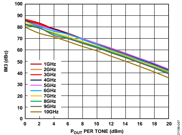
Figure 47. IM3 vs. P_{OUT} per Tone for Various Frequencies, Self Biased Mode, V_{DD} = 15 V, V_{GG1} = GND
