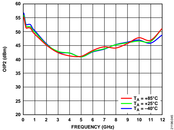
Figure 45. OIP2 vs. Frequency for Various Temperatures, P_{OUT} per Tone = 14 dBm, Self Biased, V_{DD} = 12 V, V_{GG1} = GND
