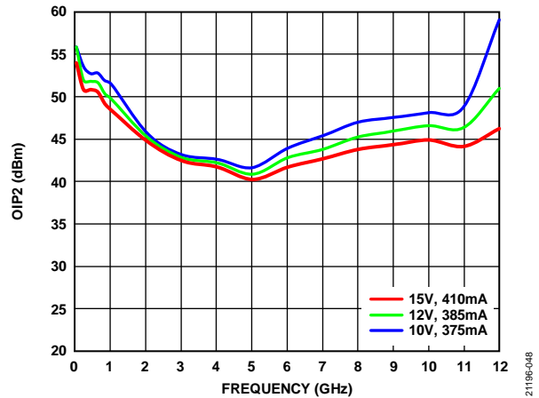
Figure 48. OIP2 vs. Frequency for Various V_{DD} and Quiescent Currents, Self Biased Mode, V_{GG1} = GND, P_{OUT} per Tone = 14 dBm
