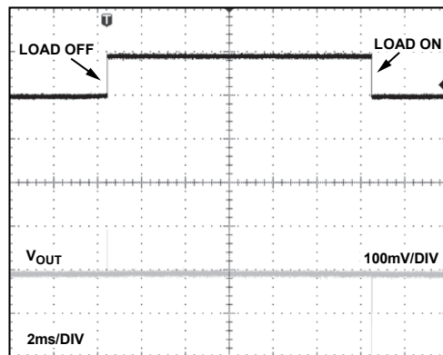
Figure 30. ADR361 Load Transient Response
