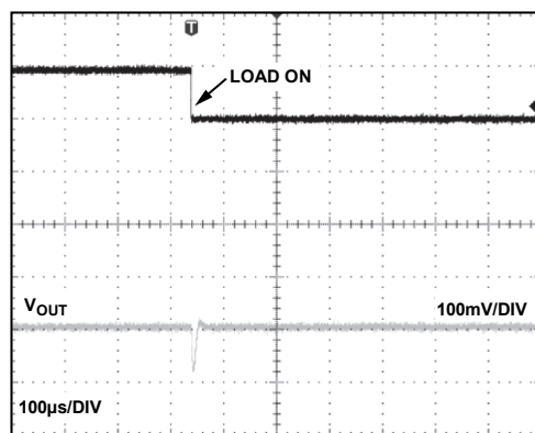
Figure 31. ADR361 Load Transient Response with 0.1 \mu\text{F} Output Capacitor
