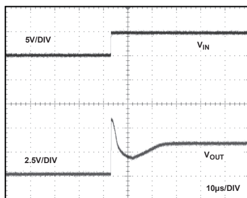
Figure 32. ADR361 Turn On Response Time at 5 V
