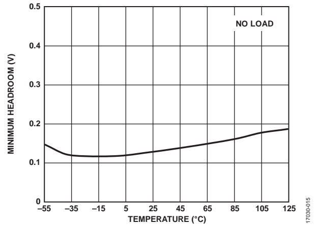
Figure 9. Minimum Headroom vs. Temperature
