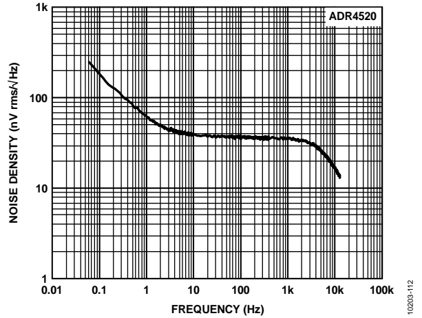
Figure 13. ADR4520 Output Noise Spectral Density
