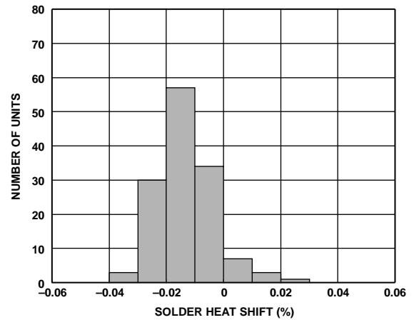
Figure 101. ADR4550 Solder Heat Resistance Shift (3 × Reflow)
