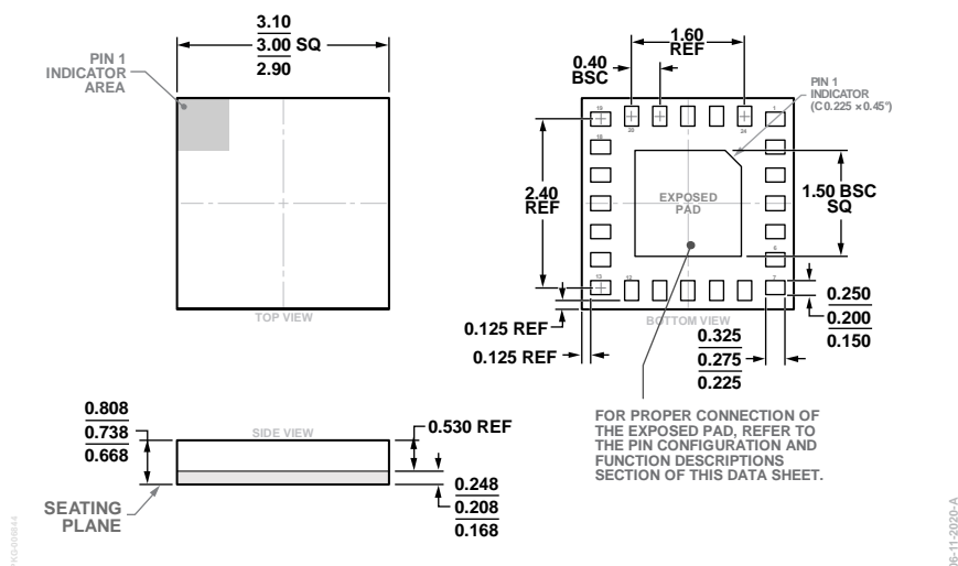
Figure 26. 24-Terminal Land Grid Array [LGA] 3 mm x 3 mm Body and 0.738 mm Package Height (CC-24-12) Dimensions shown in millimeters
