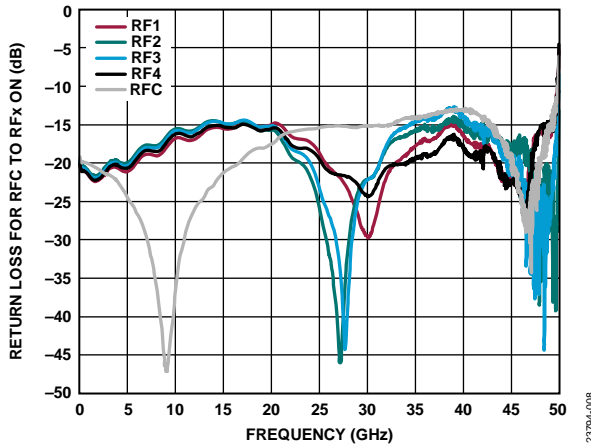
Figure 7. Return Loss for RFC and RFX On vs. Frequency
