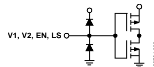
Figure 5. V1, V2, EN, and LS Pin Interface Schematic
