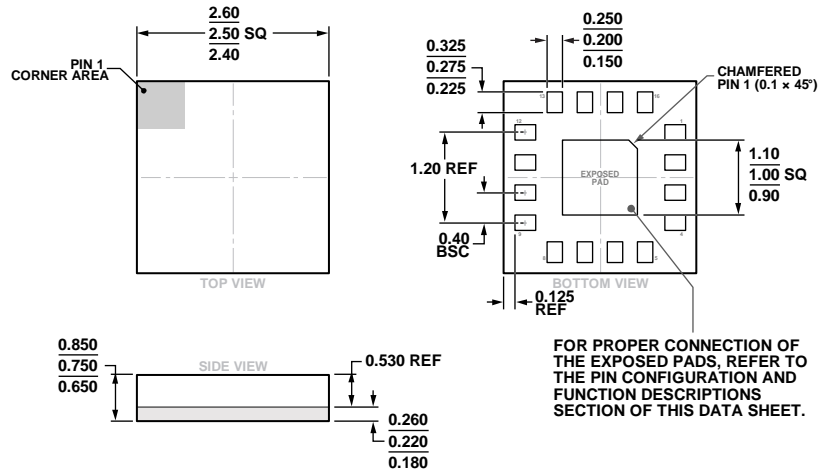
Figure 35. 16-Terminal Land Grid Array [LGA] 2.5 mm × 2.5 mm Body and 0.75 mm Package Height (CC-16-6)
