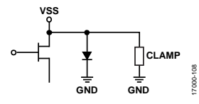
Figure 9. VSS Pin Interface Schematic
