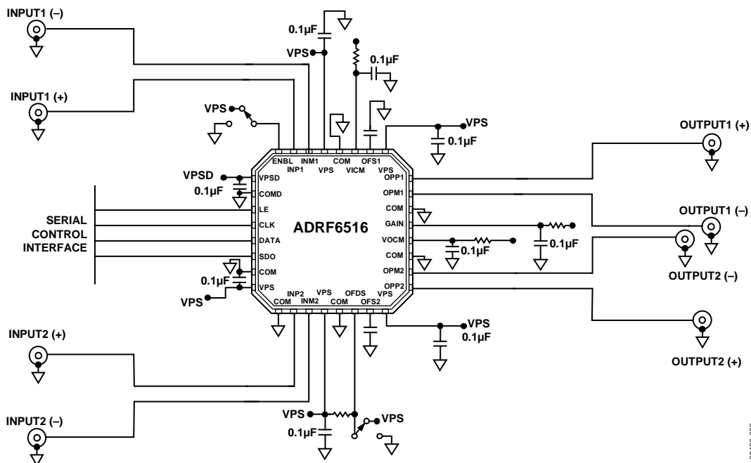
Figure 51. Basic Connections
