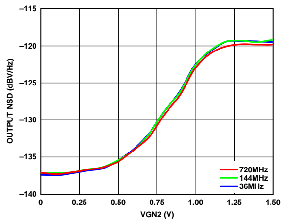
Figure 25. Output NSD vs. VGN2 for 36 MHz, 144 MHz, 720 MHz; VGN1 = 1.5 V
