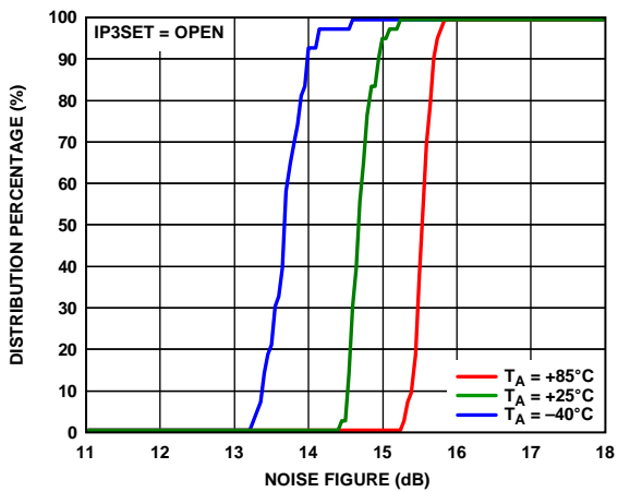
Figure 28. Noise Figure
