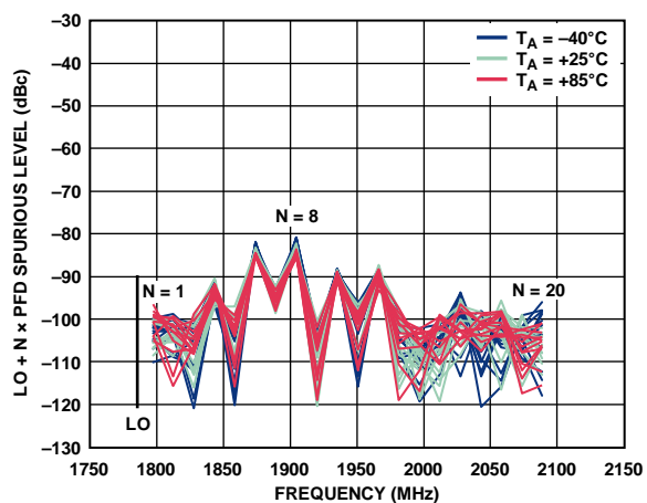
Figure 60. PFD Spurious Emissions on Modulator Output, f_{LO} + N \times f_{PFD} ; f_{LO} = 1781.76 \text{ MHz} , R_{FOUT} \approx 4 \text{ dBm} at 25^\circ\text{C} , f_{REF} = 61.44 \text{ MHz} at 4 \text{ dBm} , f_{PFD} = 15.36 \text{ MHz} , Integer PLL Mode
