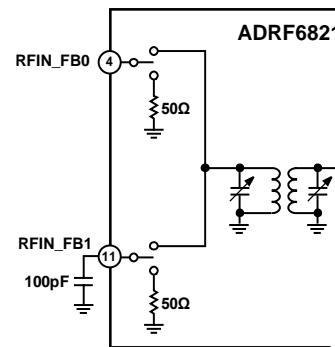
Figure 45. Terminating the Unused Port of the ADRF6821
