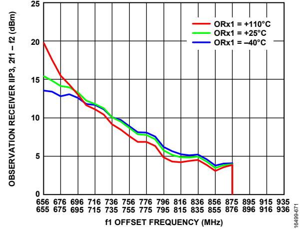
Figure 168. Observation Receiver IIP3, 2f_1 - f_2 vs. f_1 Offset Frequency, LO = 650 MHz, Attenuation = 0 dB, Tones Separated by 1 MHz Swept Across Pass Band at -19 dBm Each
