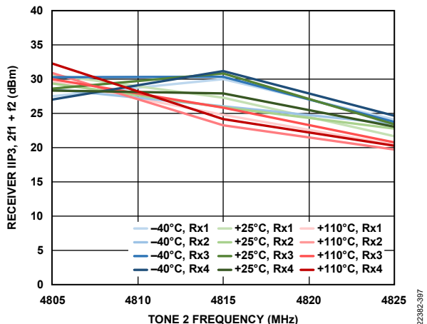
Figure 468. Receiver IIP3, 2f_1 + f_2 vs. Tone 2 Frequency, Both Tones at -11 dBFS, f_1 = f_2 + 2 MHz
