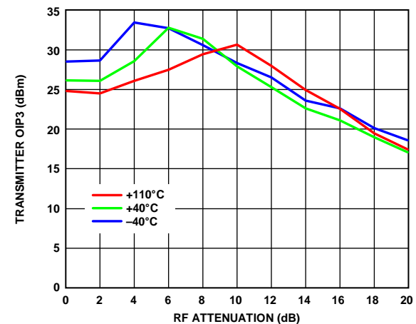
Figure 34. Transmitter OIP3 vs. RF Attenuation, 800 MHz LO, 20 MHz RF Bandwidth, f_1 = 10 MHz, f_2 = 11 MHz, 3 dB Digital Backoff, 122.88 MSPS Sample Rate
