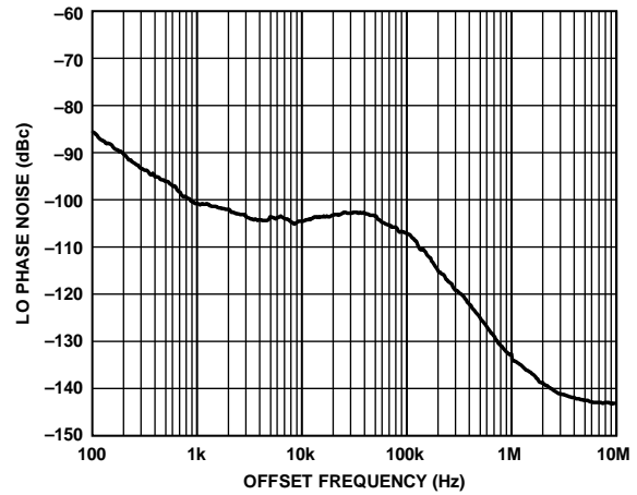
Figure 32. LO Phase Noise vs. Offset Frequency, 3 dB Digital Backoff, 710 MHz LO
