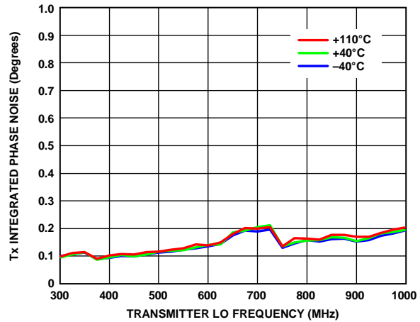
Figure 33. Tx Integrated Phase Noise vs. Transmitter LO Frequency, 20 MHz RF Bandwidth, CW 20 MHz Offset from LO, 3 dB Digital Backoff
