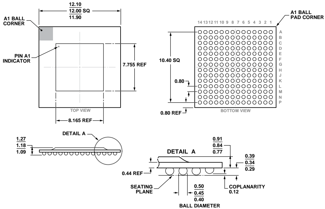
COMPLIANT TO JEDEC STANDARDS MO-275-GGAB-1. Figure 234. 196-Ball Chip Scale Package Ball Grid Array [CSP_BGA] (BC-196-12) Dimensions shown in millimeters
