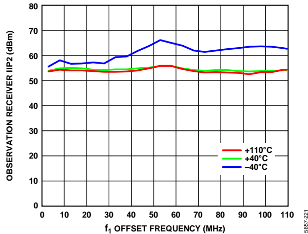
Figure 221. Observation Receiver IIP2 vs. f_1 Offset Frequency, 5600 MHz LO, 0 dB Attenuation, 200 MHz RF Bandwidth, f_2 = f_1 + 1 MHz, 245.76 MSPS Sample Rate
