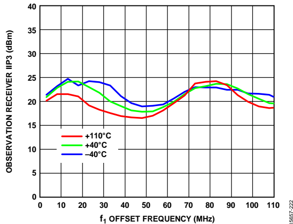
Figure 223. Observation Receiver IIP3 vs. f_1 Offset Frequency, 5600 MHz LO, 0 dB Attenuation, 200 MHz RF Bandwidth, f_2 = 2f_1 + 1 MHz, 245.76 MSPS Sample Rate
