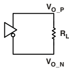
Figure 14. Link Ports—Transmit Electrical Characteristics
