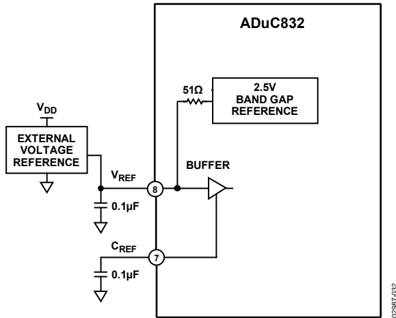
Figure 43. Using an External Voltage Reference
