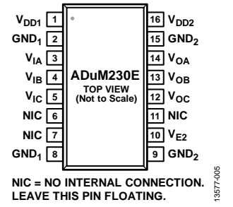
Figure 7. ADuM230E Pin Configuration
