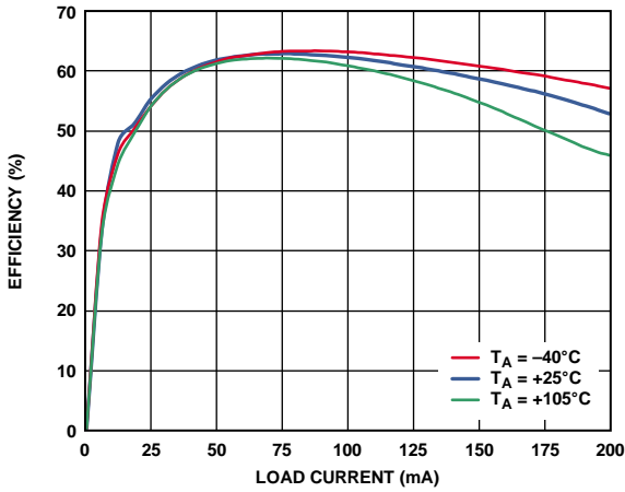
Figure 10. Typical Efficiency over Temperature with 1:3 Coilcraft Transformer (CR7984-CL), f_{SW} = 500 kHz, 3.3 V Input to 5 V Output
