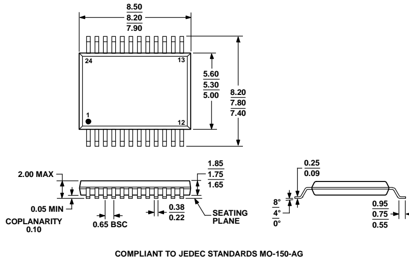
COMPLIANT TO JEDEC STANDARDS MO-150-AG Figure 35. 24-Lead Shrink Small Outline Package [SSOP] (RS-24) Dimensions shown in millimeters
