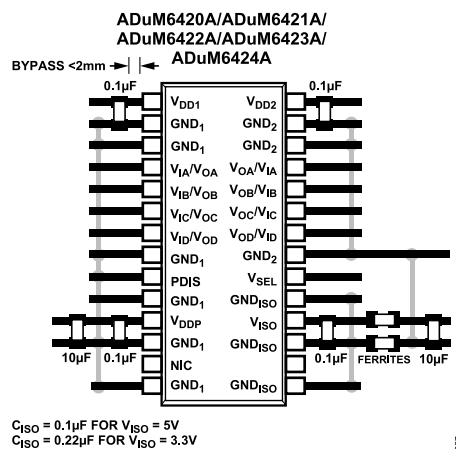
Figure 25. Recommended PCB Layout
