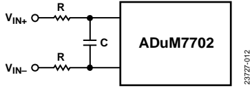
Figure 30. Differential RC Filter Network
