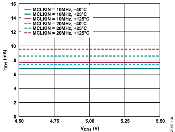
Figure 20. I_{DD1} vs. V_{DD1} at Clock Rates and Various Temperatures
