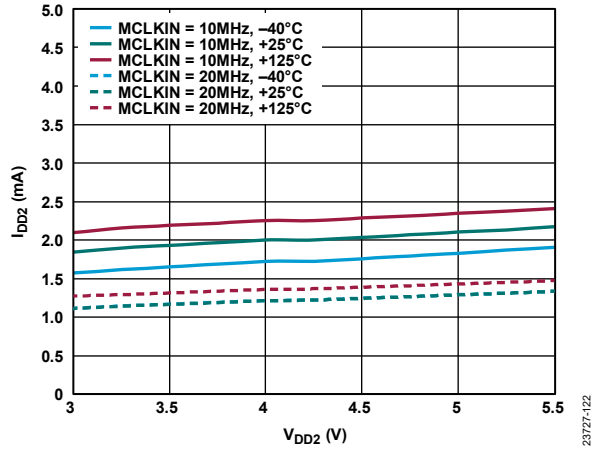
Figure 22. I_{DD2} vs. V_{DD2} at Various Clock Rates and Temperatures
