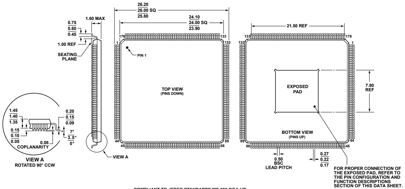
Figure 108. 176-Lead Low Profile Quad Flat Package [LQFP_EP] (SW-176-1) Dimensions shown in millimeters
